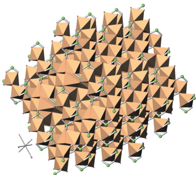
Fig. 2 Structure of \text{Sr}_4[\text{MoN}_4]\text{O} as a projection on the [111] plane, showing the isolated \text{MoN}_4 tetrahedra (ball and stick representation) within the cavities of the \text{Sr}-(\text{N},\text{O}) framework (polyhedra).
